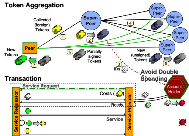
Figure 1: Token-Accounting-System
