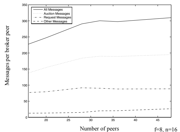
Figure 3. Message Overhead
